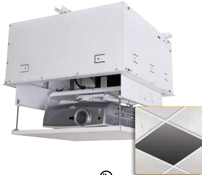
Now fits into 2' x 2' (600 x 600 mm) ceiling tile, with up to 8.5" (216 mm) extension
